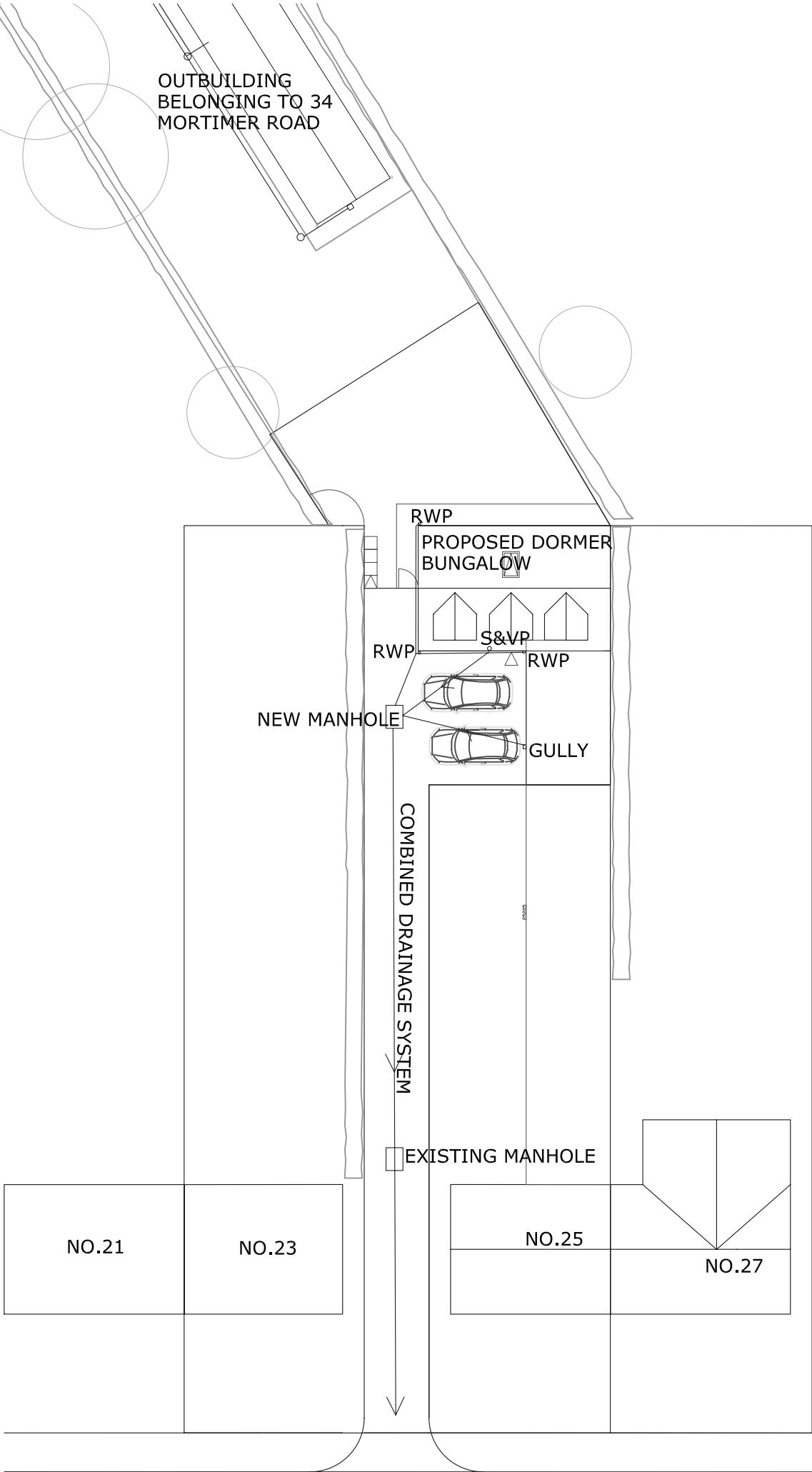
PROPOSED SITE LAYOUT
