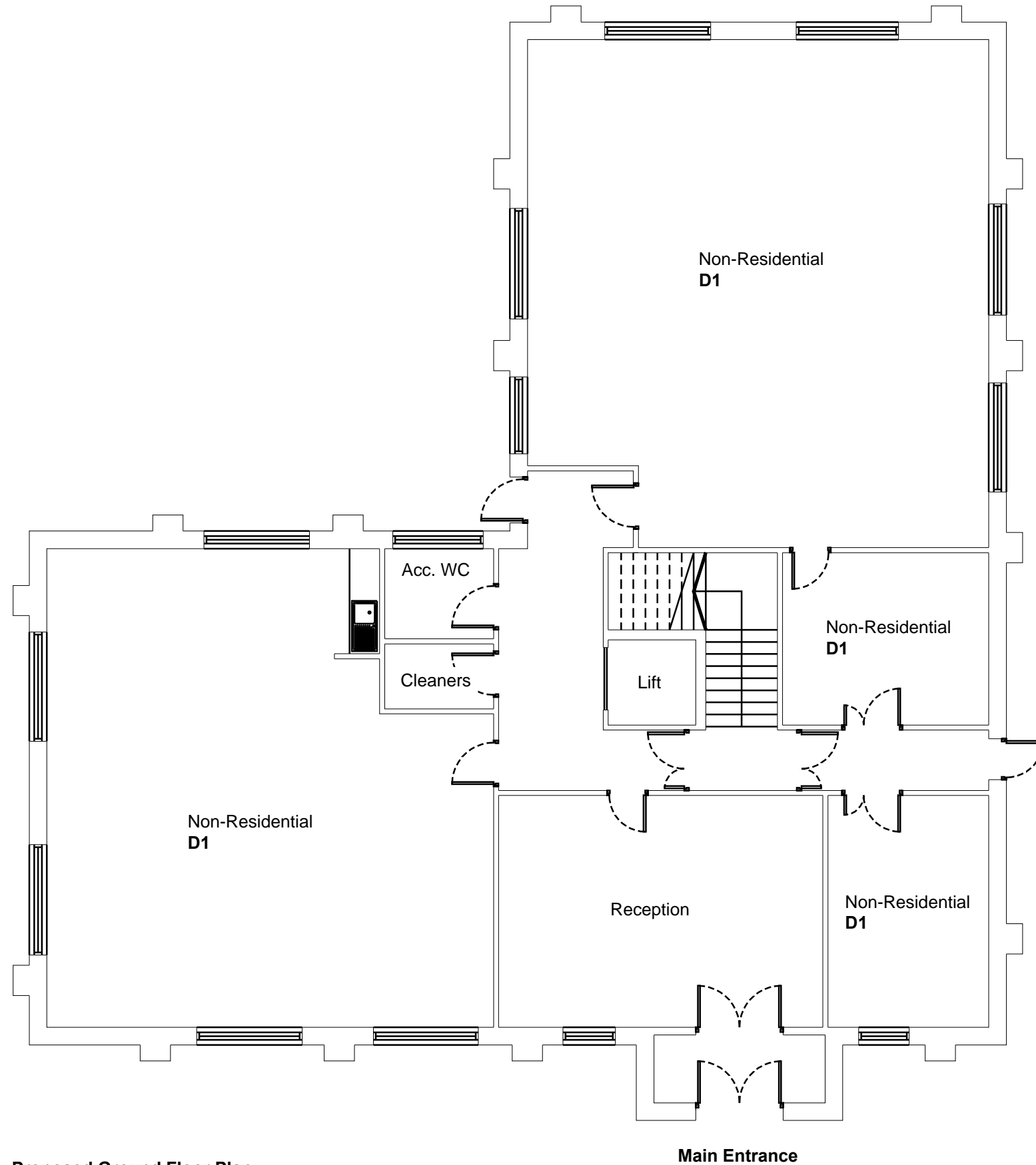
Proposed Ground Floor Plan Phoenix House Tankersley
