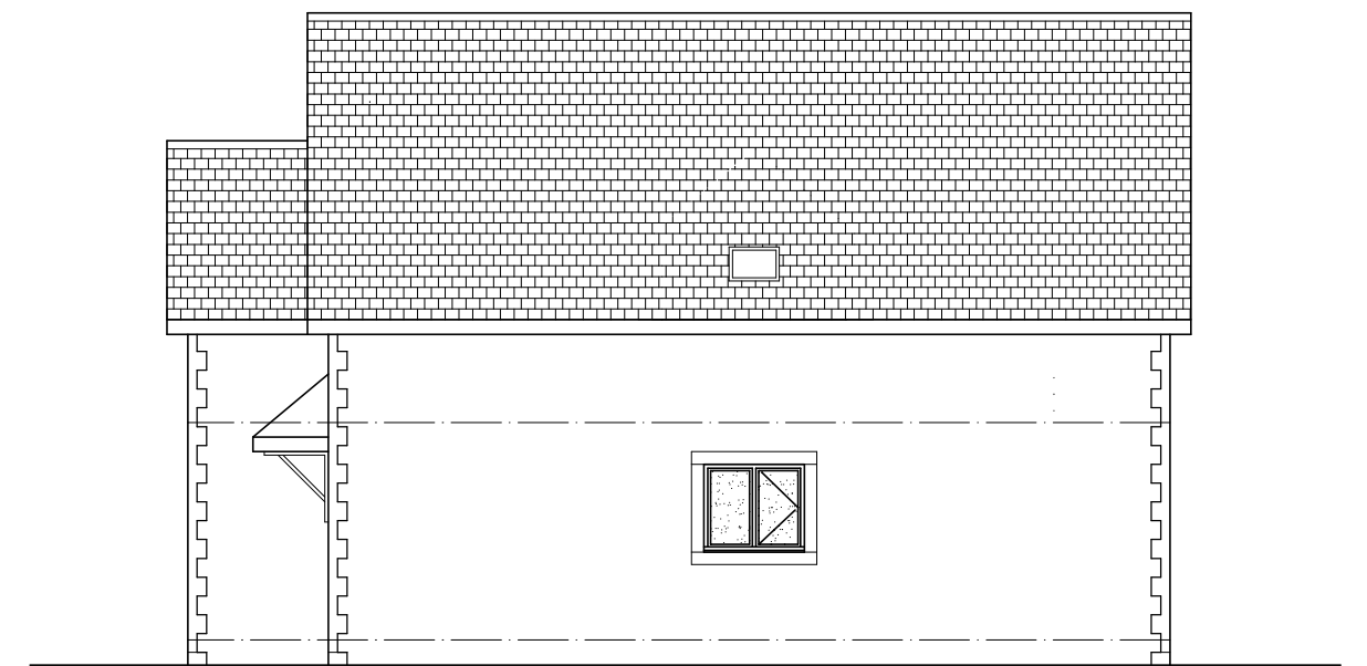
SIDE ELEVATION
