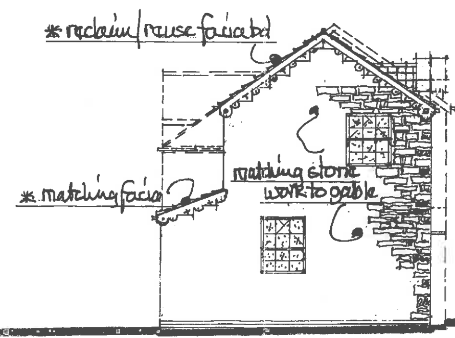
proposed gable view.
