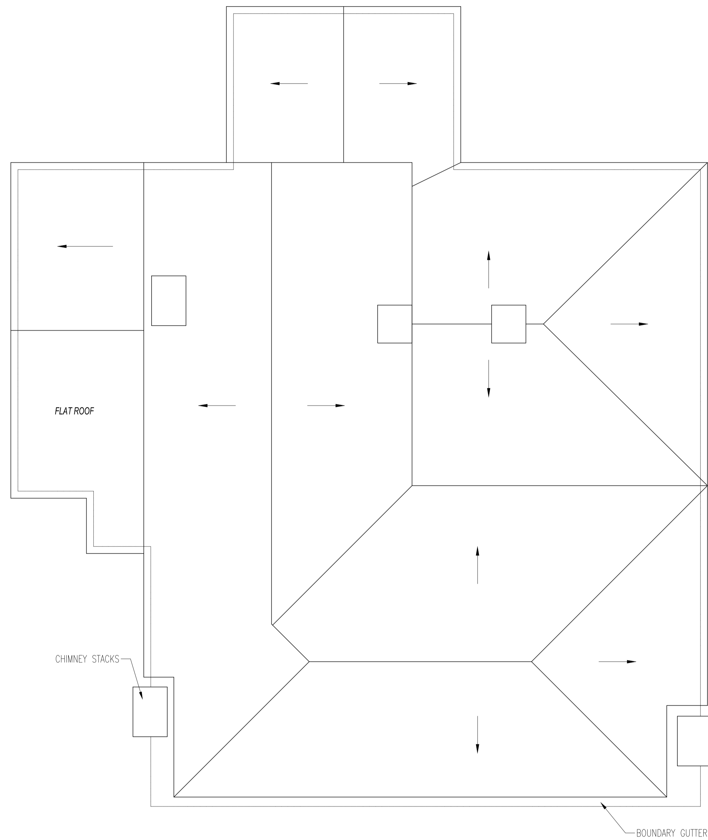
EXISTING ROOF PLAN SCALE 1:50
