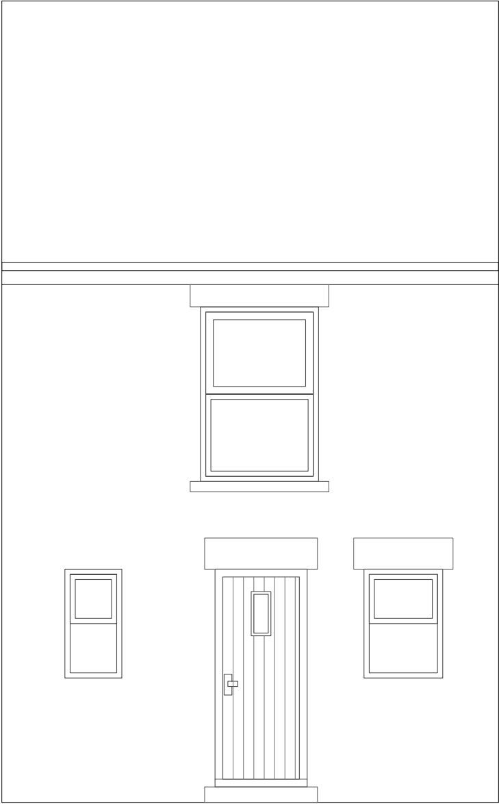
EXISTING REAR ELEVATION TO COURTYARD
