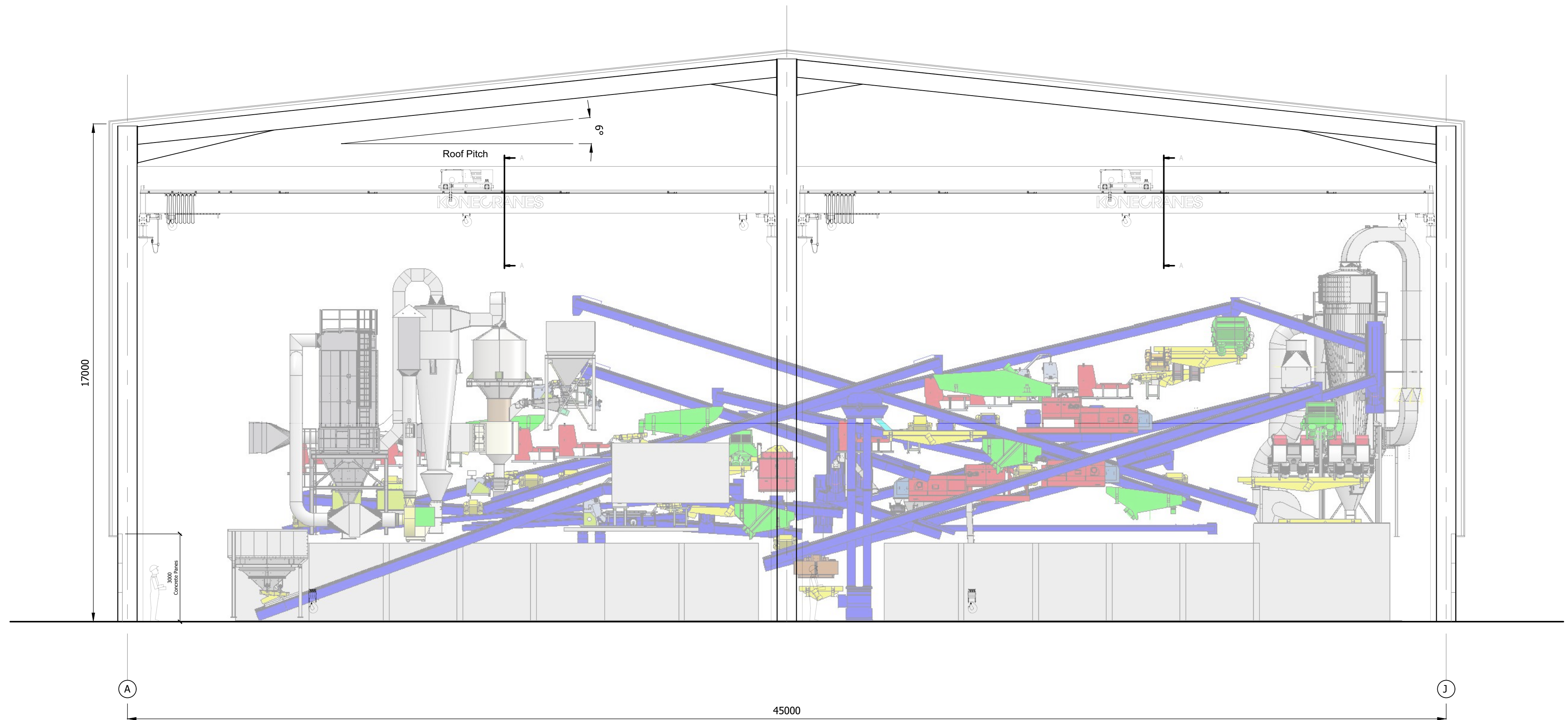
Proposed Typical Section Scale 1 : 100
