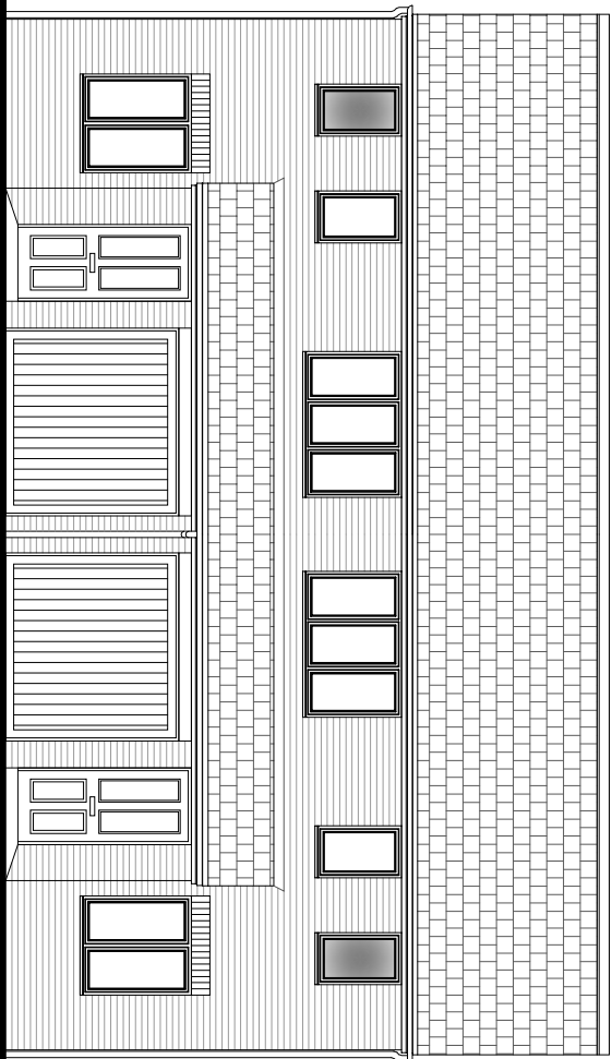
Front Elevation
