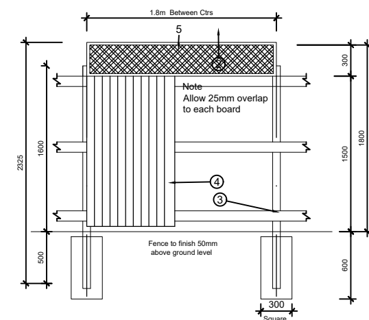
1500mm High Timber Close Boarded Fence with 300mm High Trellis (16)
