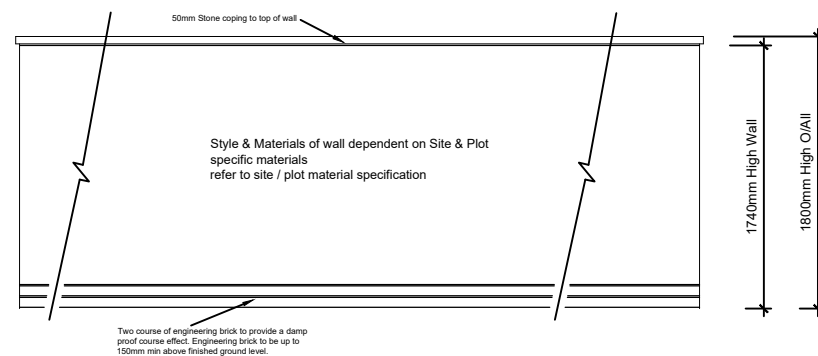
1800mm High Screen Wall 225mm Thick (2)
