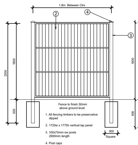
1800mm High Vertical Panel Fence (4)
