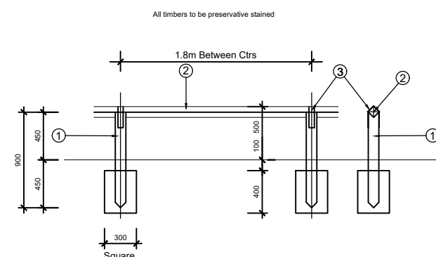
Low Trip Fence (12)
