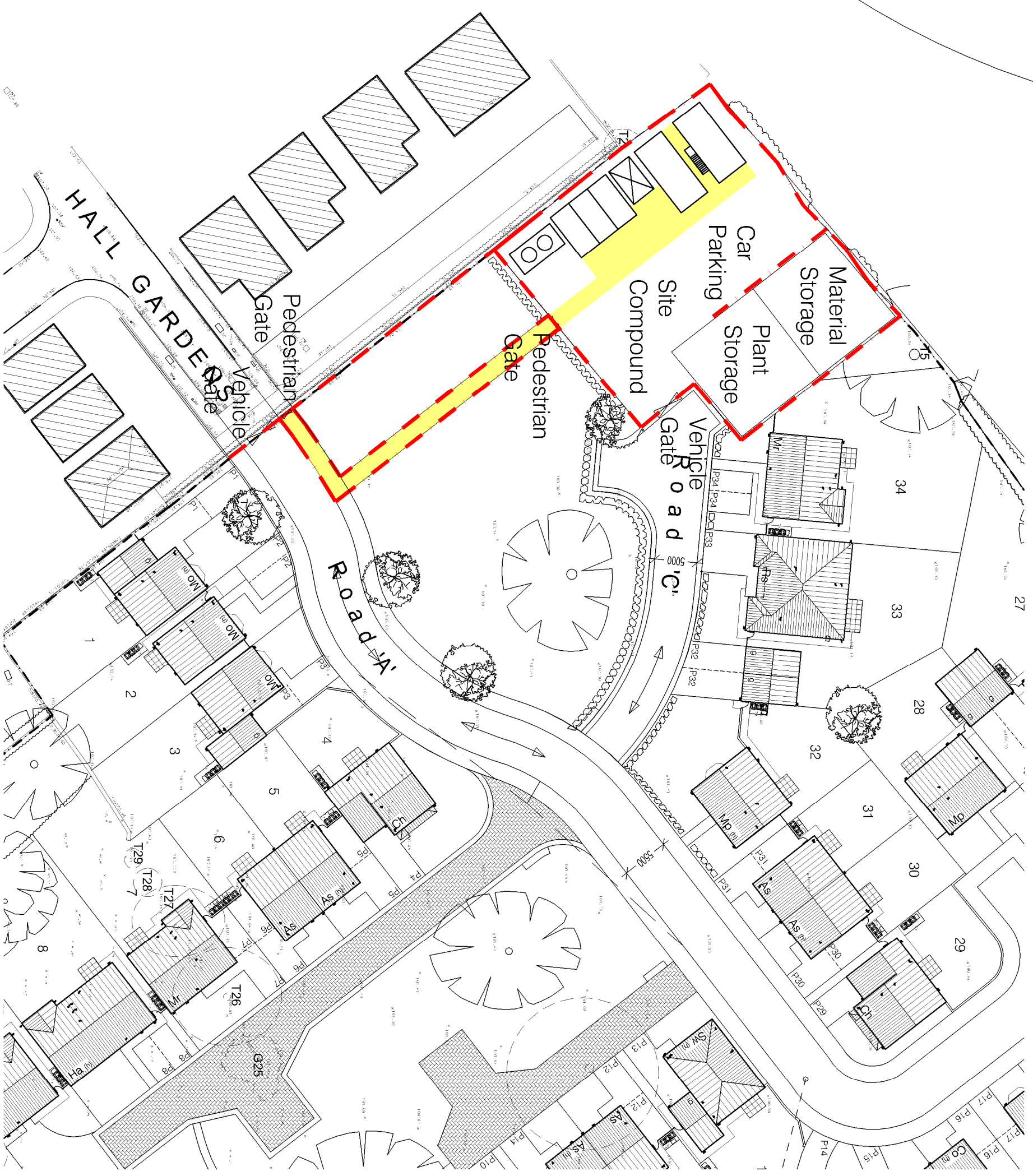
Site Layout Plan 1:500
