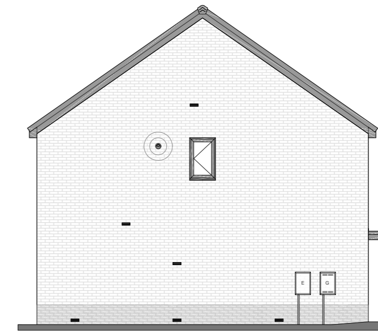
LEFT ELEVATION
