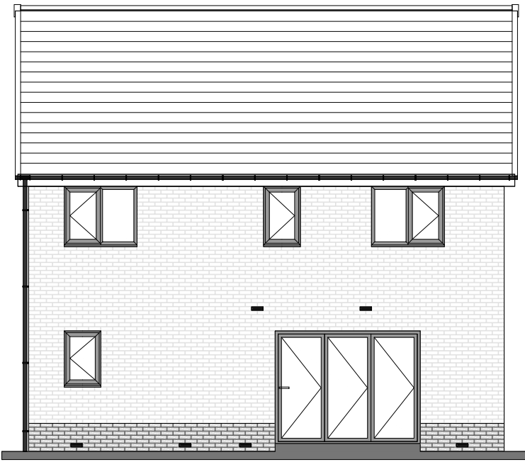
REAR ELEVATION
