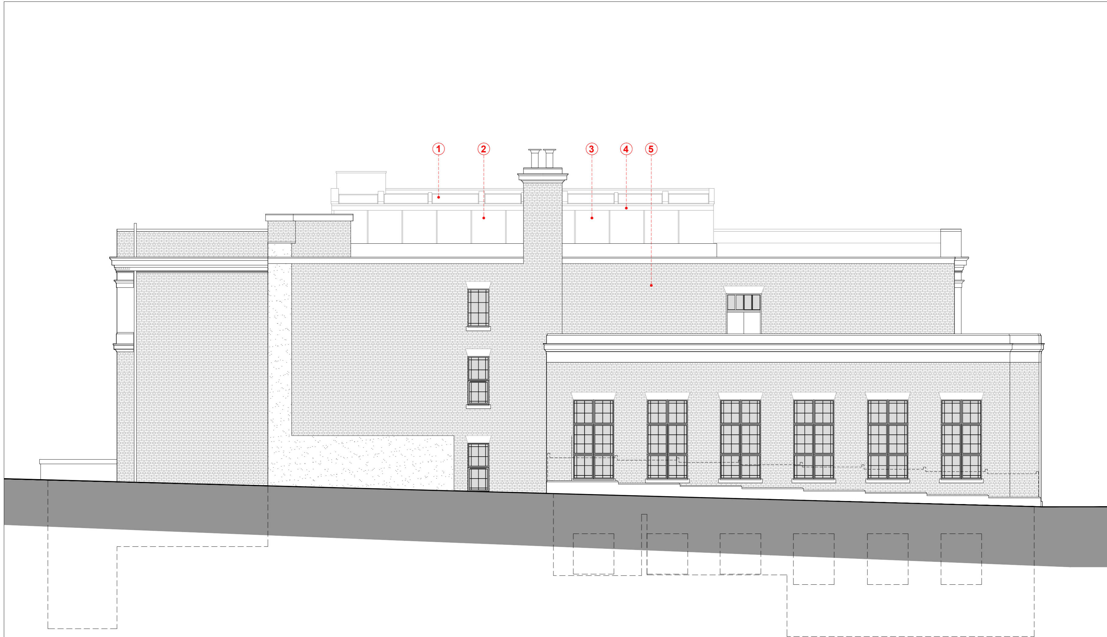
PROPOSED ELEVATION D (REAR) 1:100 @ A1
