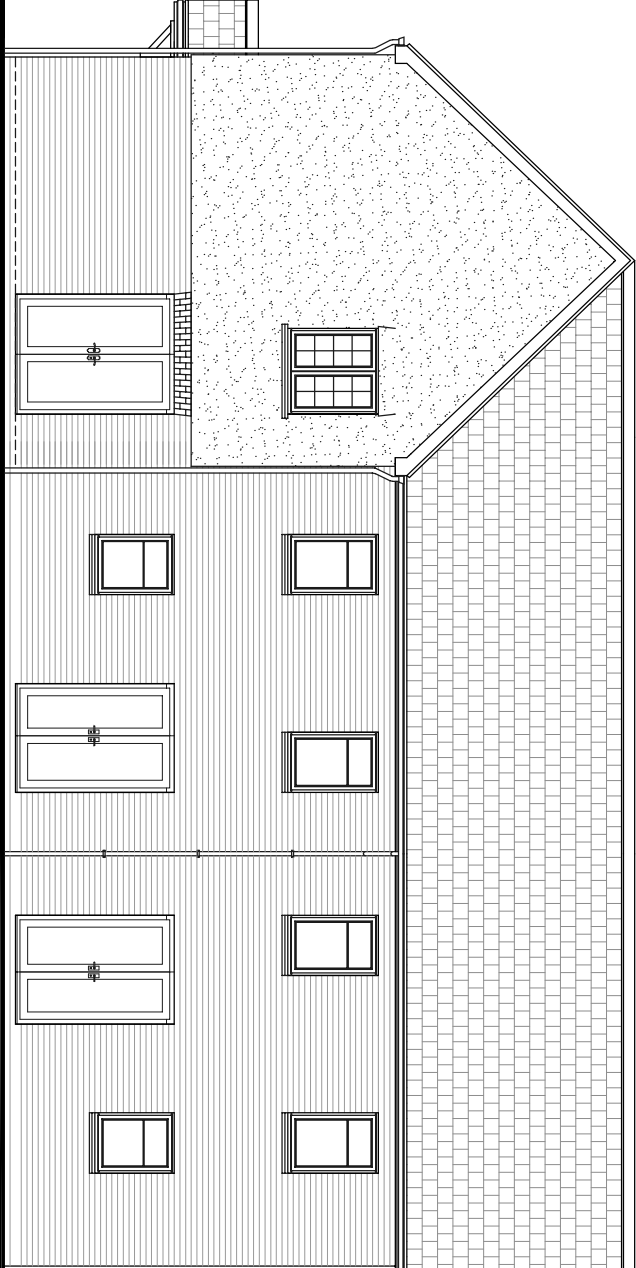
REAR ELEVATION
