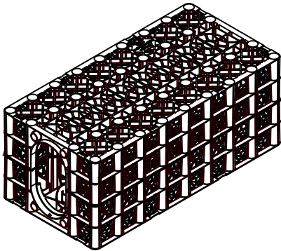
ISOMETRIC VIEW Scale 1:10
