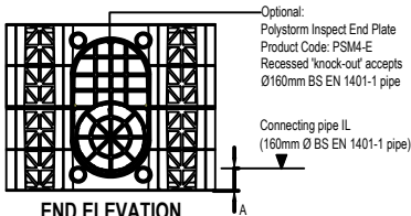
END ELEVATION (Including Insert) Scale 1:10
