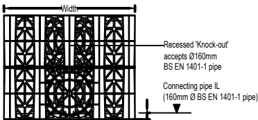
END ELEVATION Scale 1:10
