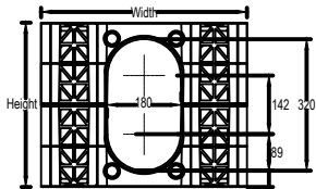
END ELEVATION Scale 1:10
