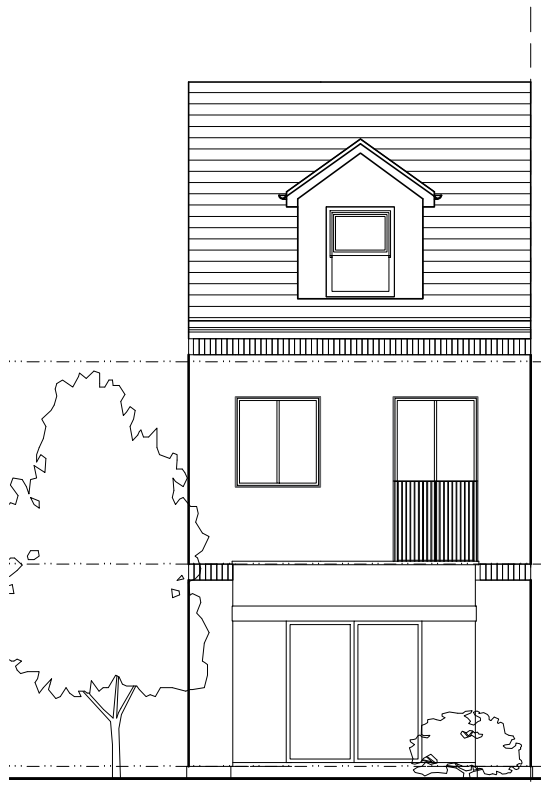
REAR ELEVATION
