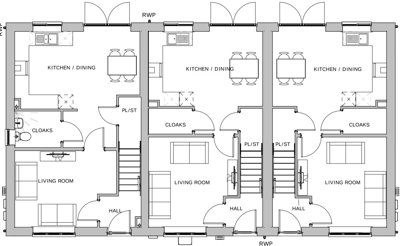
Ground Floor 1 : 100
