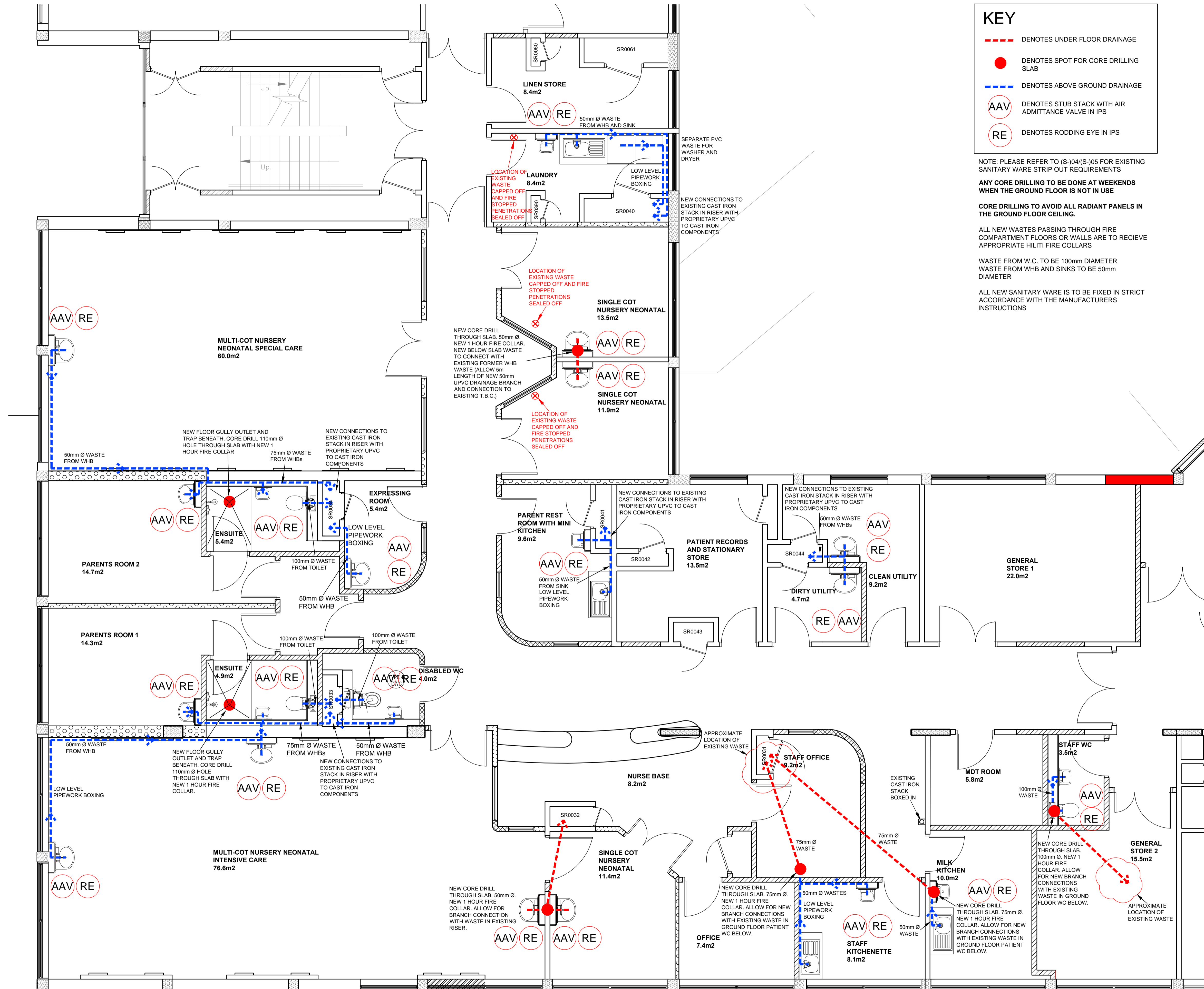
PROPOSED NEONATAL UNIT DRAINAGE PLAN 1:50
