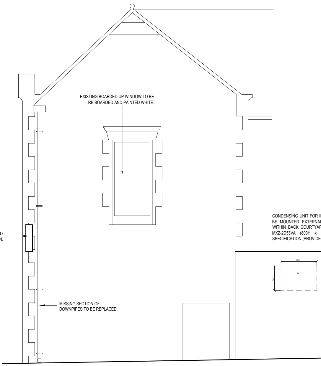
SECTION AA - 1:50
