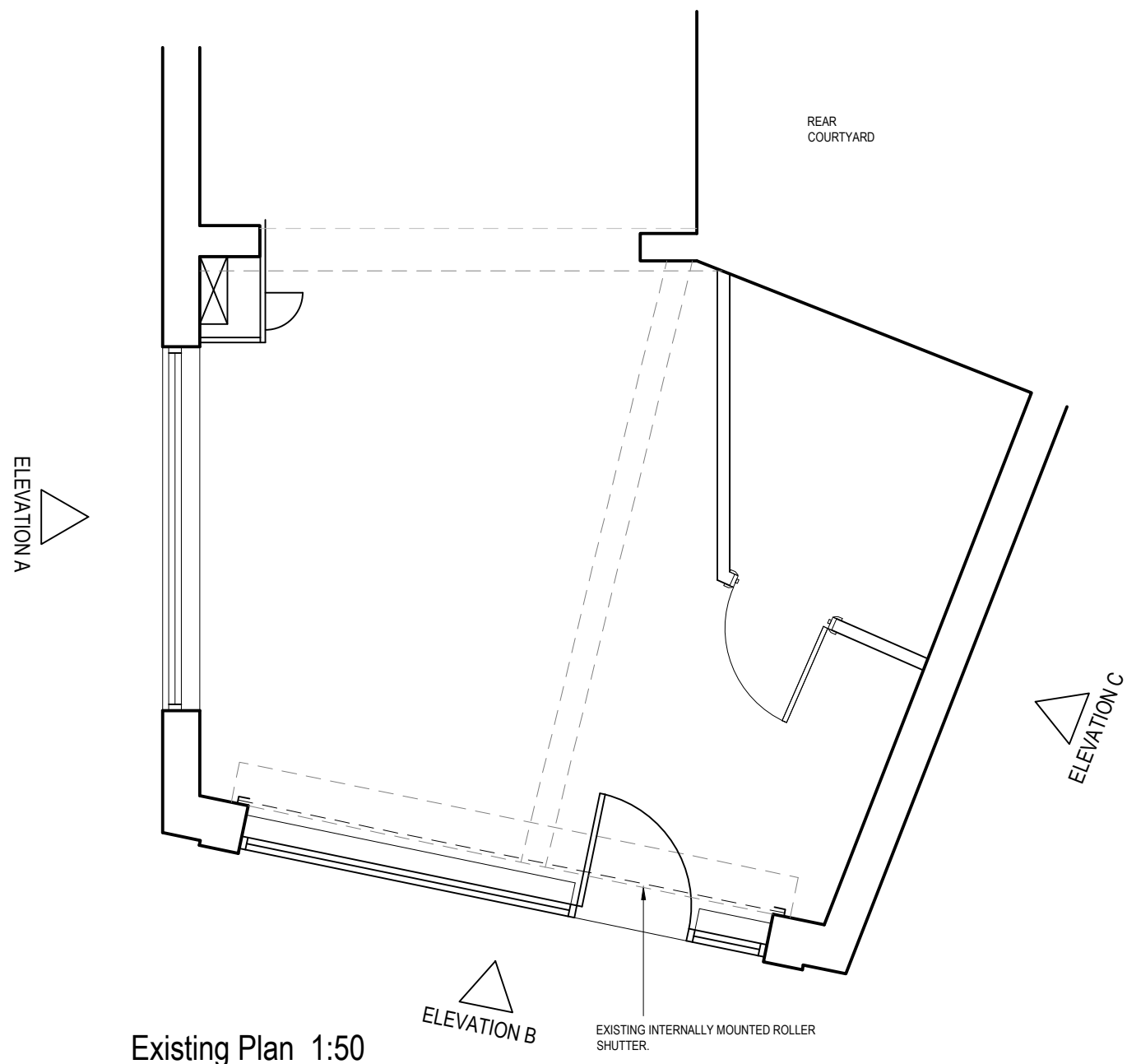
Existing Plan 1:50
