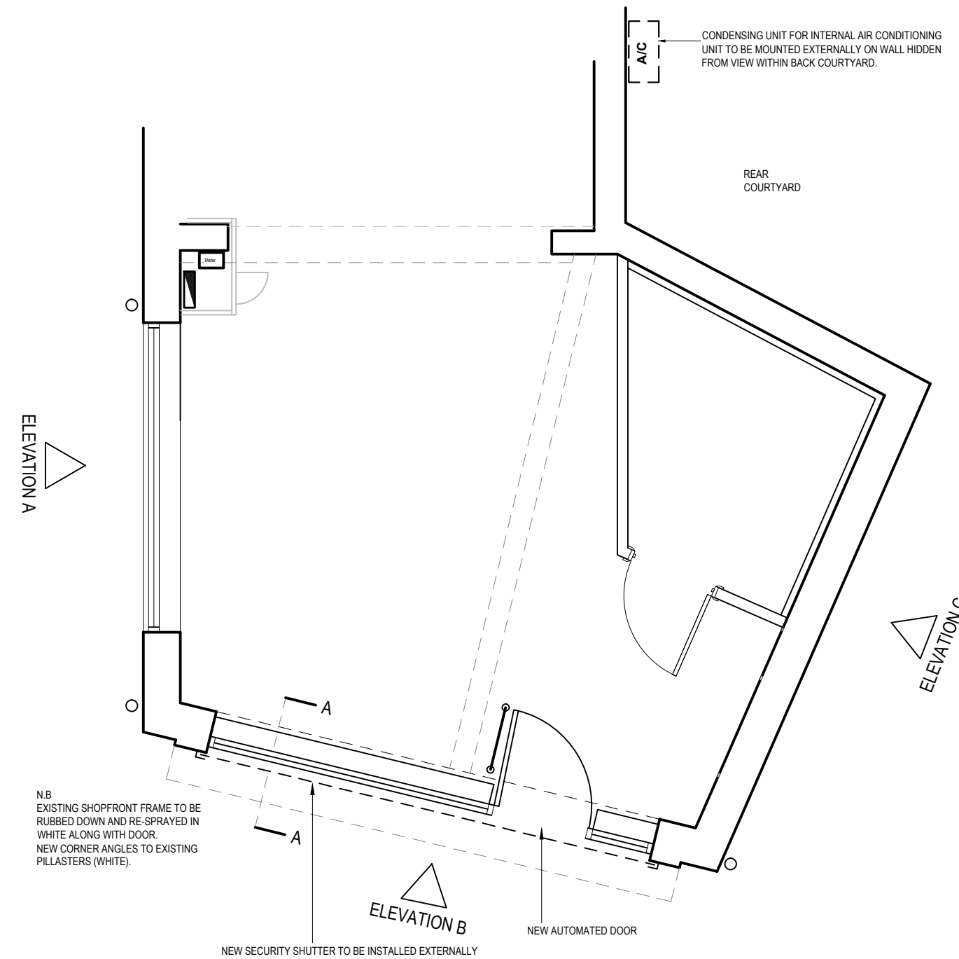
Proposed Plan 1:50
