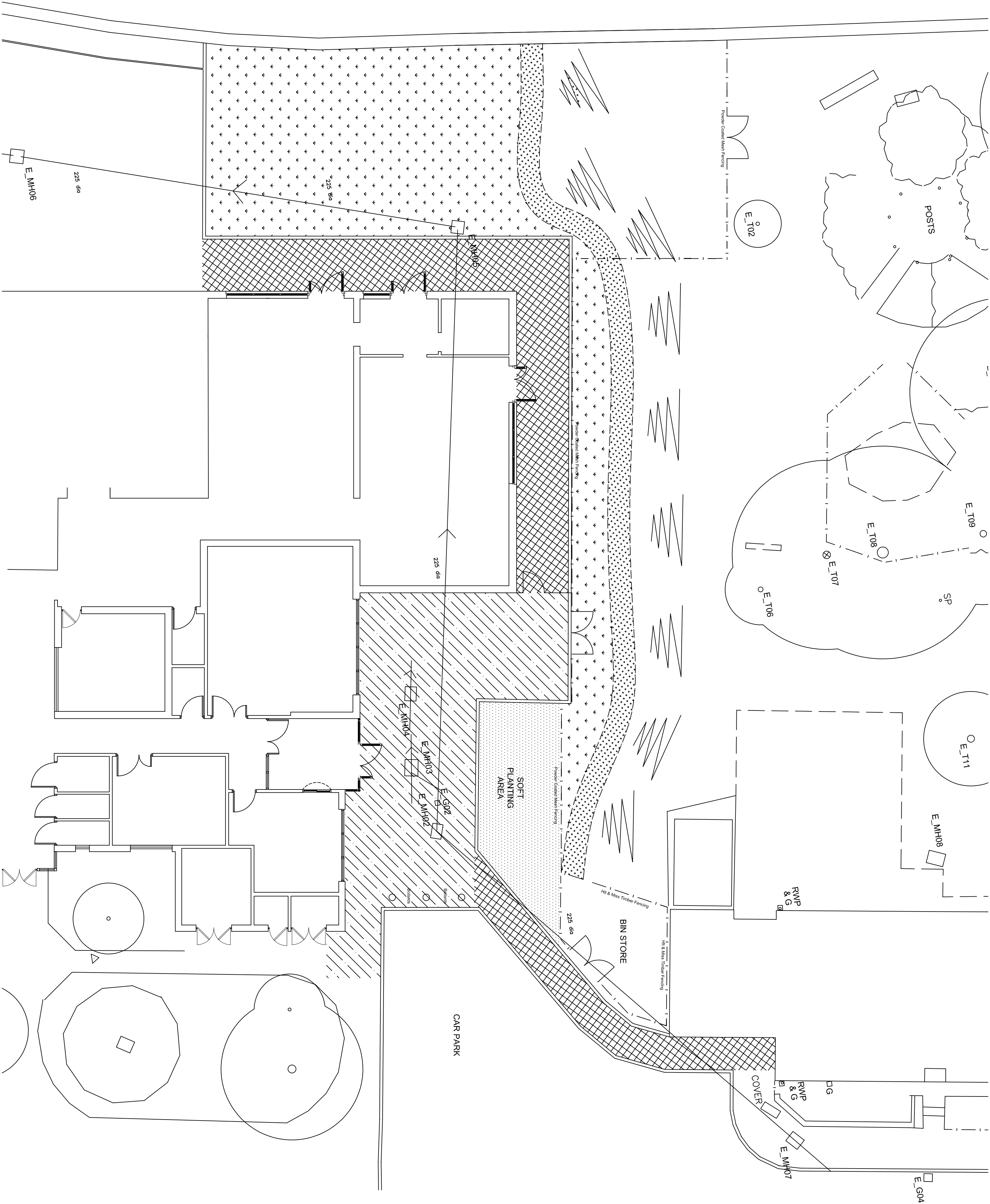
Proposed External Works Plan Scale: 1 : 100 @ A1
