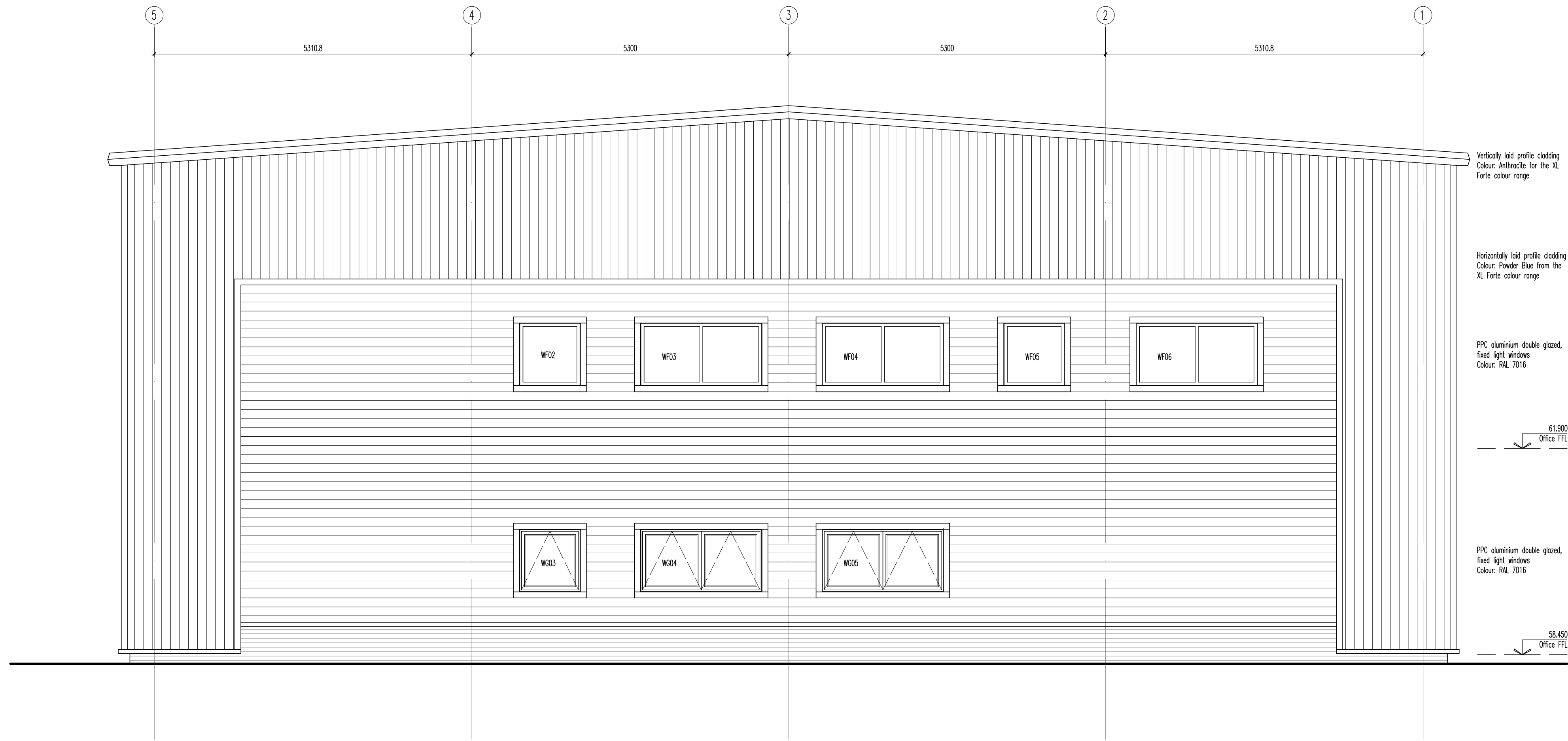
PROPOSED GABLE ELEVATION 1:500/60
