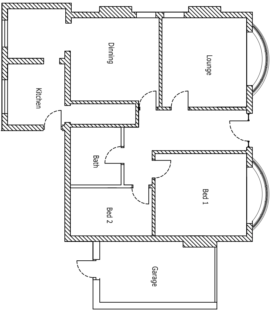
EXISTING FLOOR PLAN SCALE 1:100
