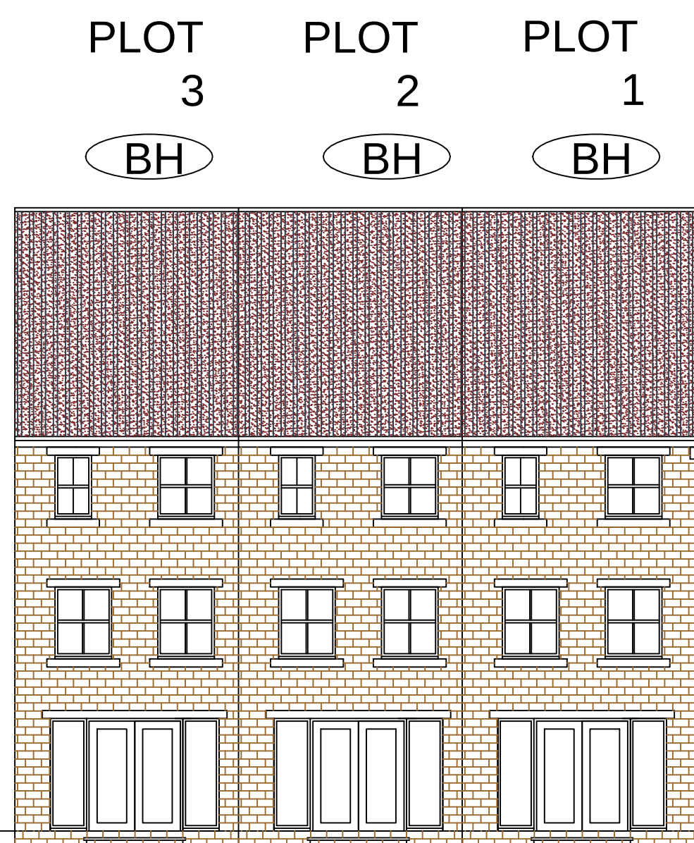
EAST ELEVATION TO PLOTS 1-3
