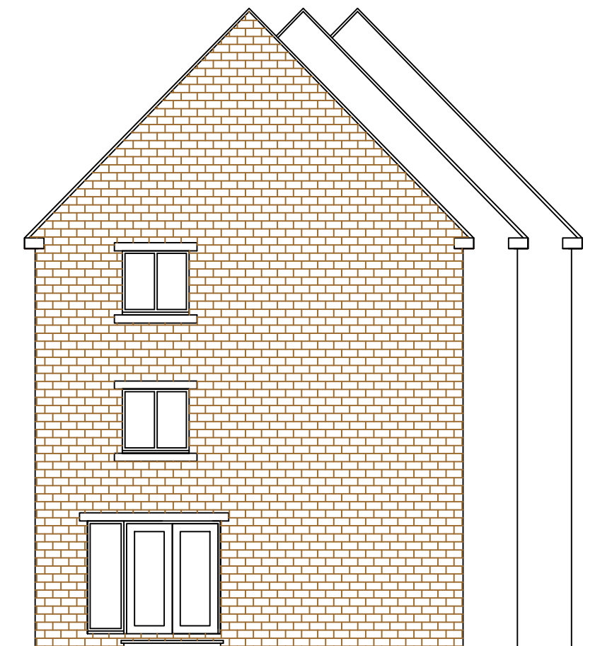
SIDE ELEVATION TYPE C
