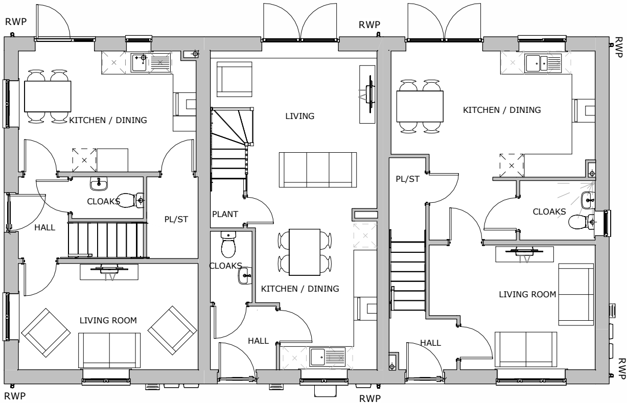
Ground Floor 1 : 100
