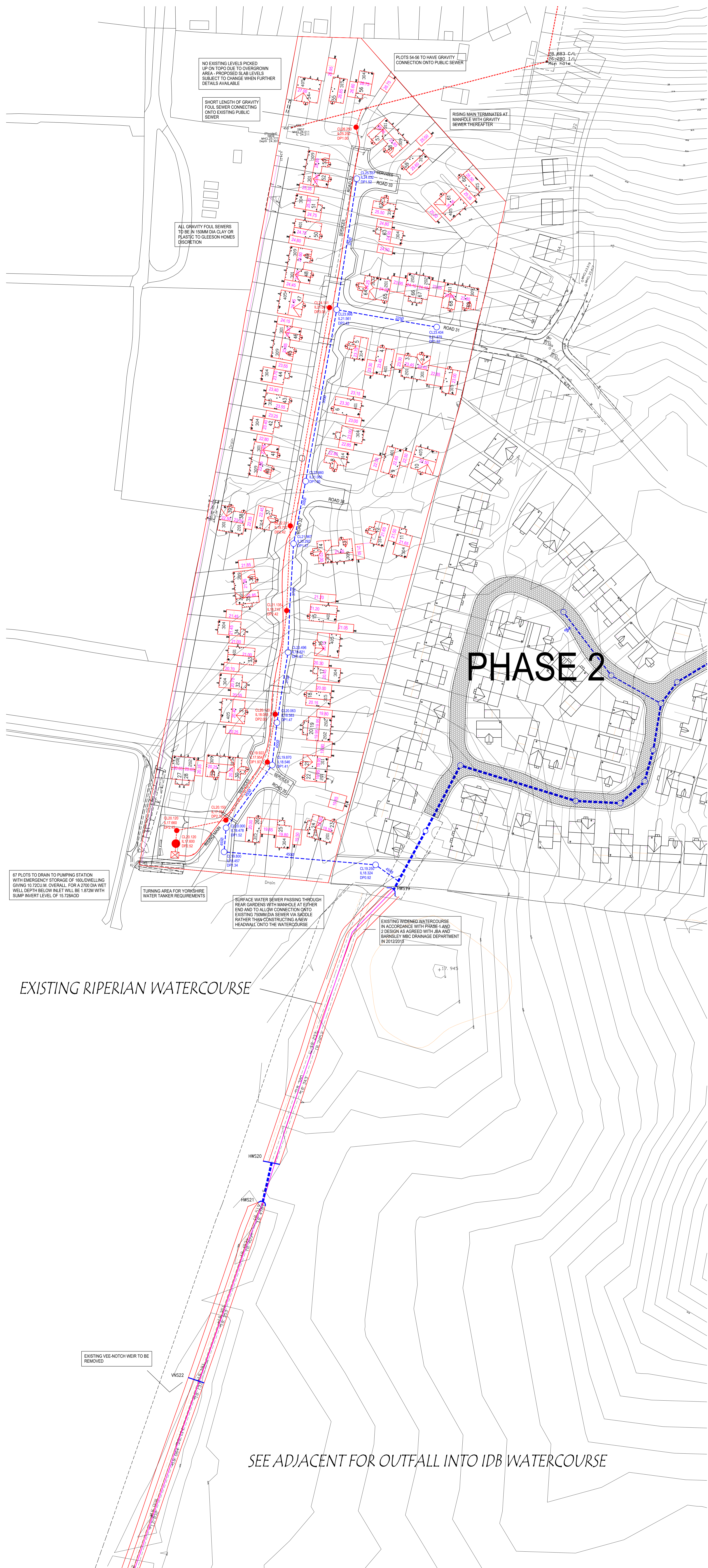
OUTFALL INTO EXISTING RIPERIAN WATERCOURSE
