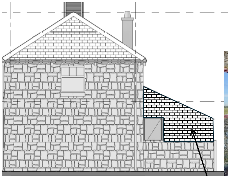
East Side Elevation - Existing
