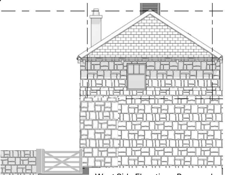
West Side Elevation - Proposed
