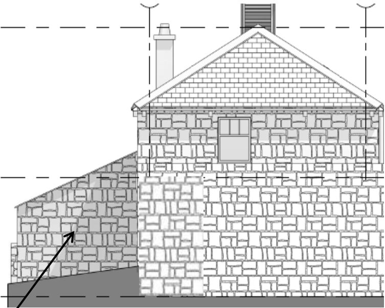
West Side Elevation - Existing
