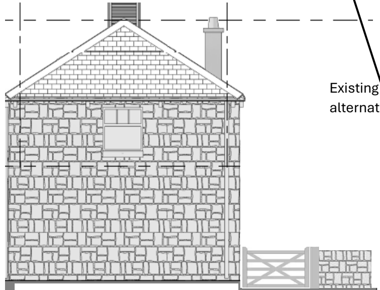
East Side Elevation - Proposed
