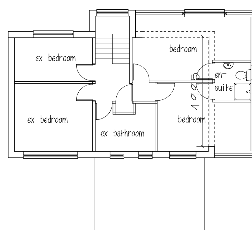
FIRST FLOOR
