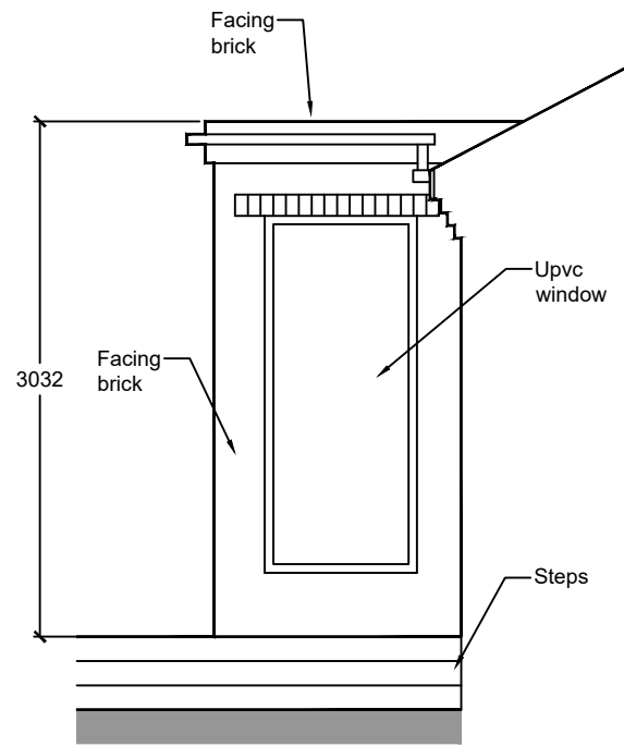
EXISTING SIDE ELEVATION 1:50
