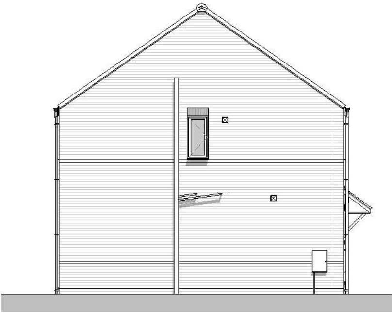
Left Side Elevation 1 : 100
