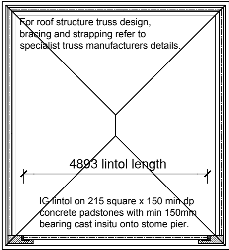
Roof Plan 1:100 Concrete pad stone to be faced in brickwork to garage door reveals
