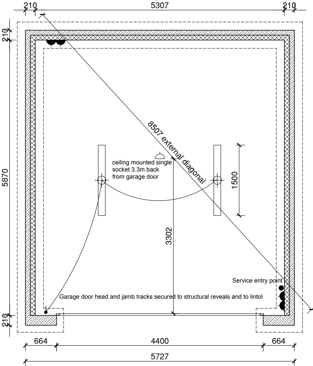
Foundation Plan 1:50
