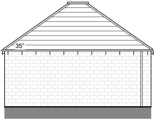
Side Elevation 1:100
