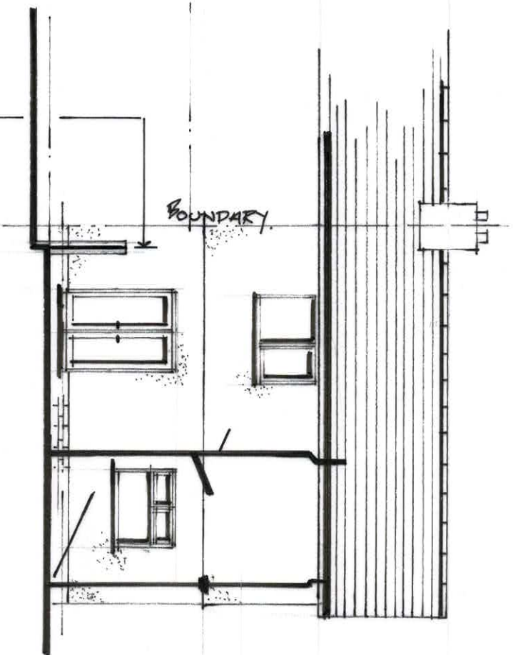
Rear Elevation
