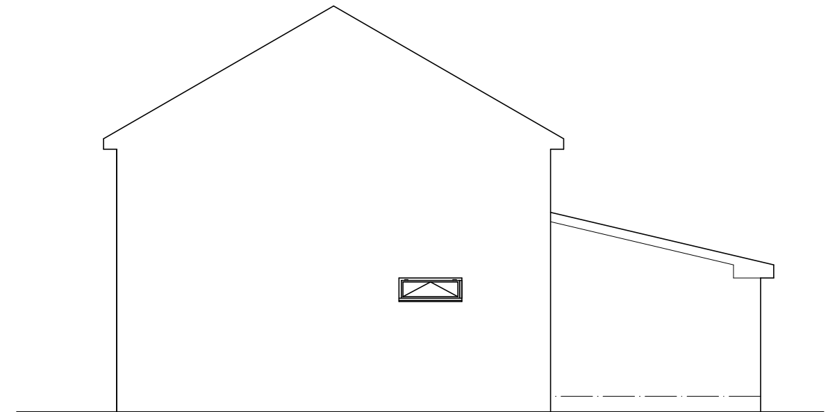
SIDE ELEVATION
