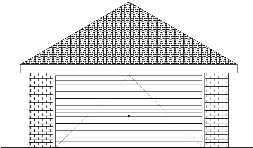
2 GARAGE FRONT ELEVATION 1 : 50
