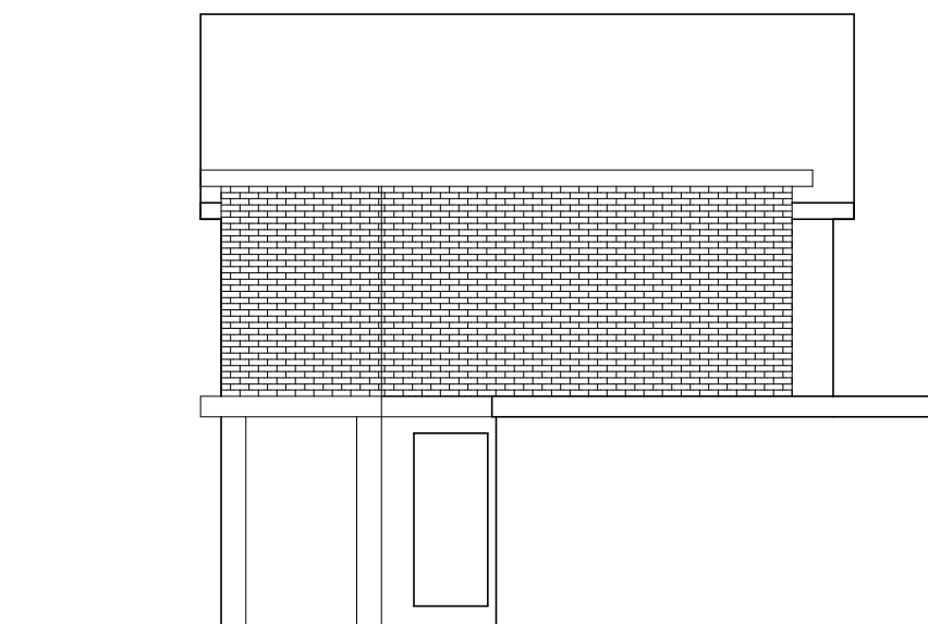
SIDE ELEVATION
