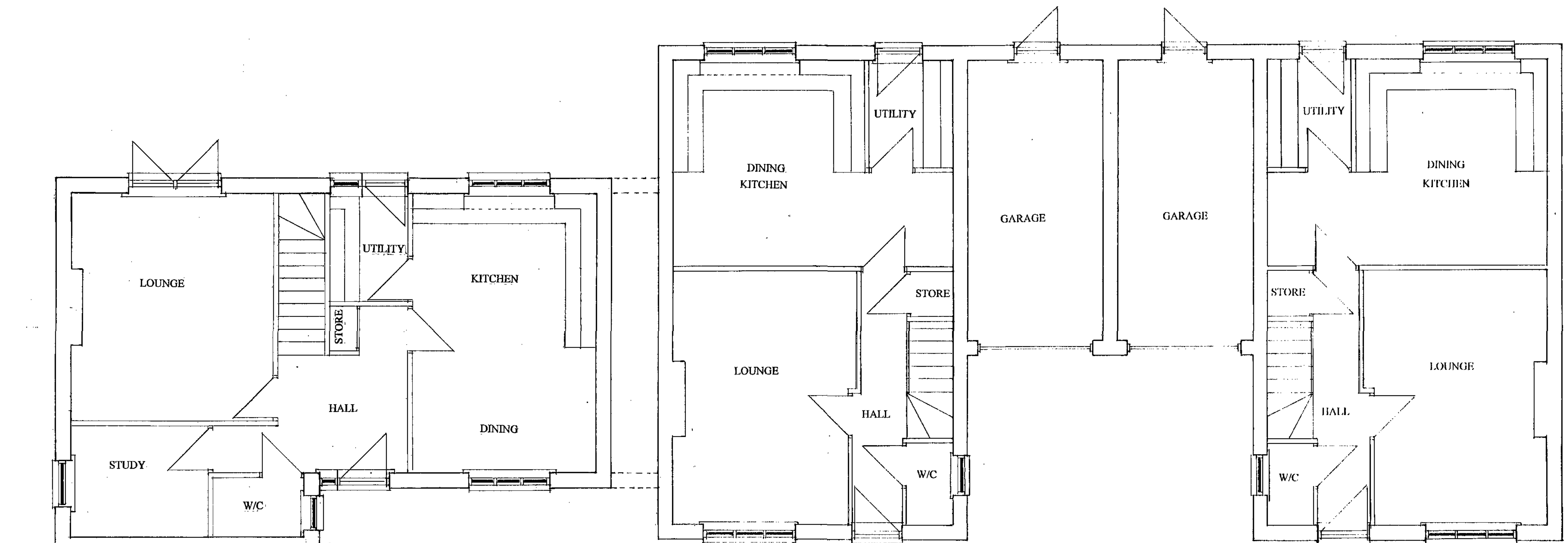
PROPOSED GROUND FLOOR LAYOUTS SCALE 1:50
