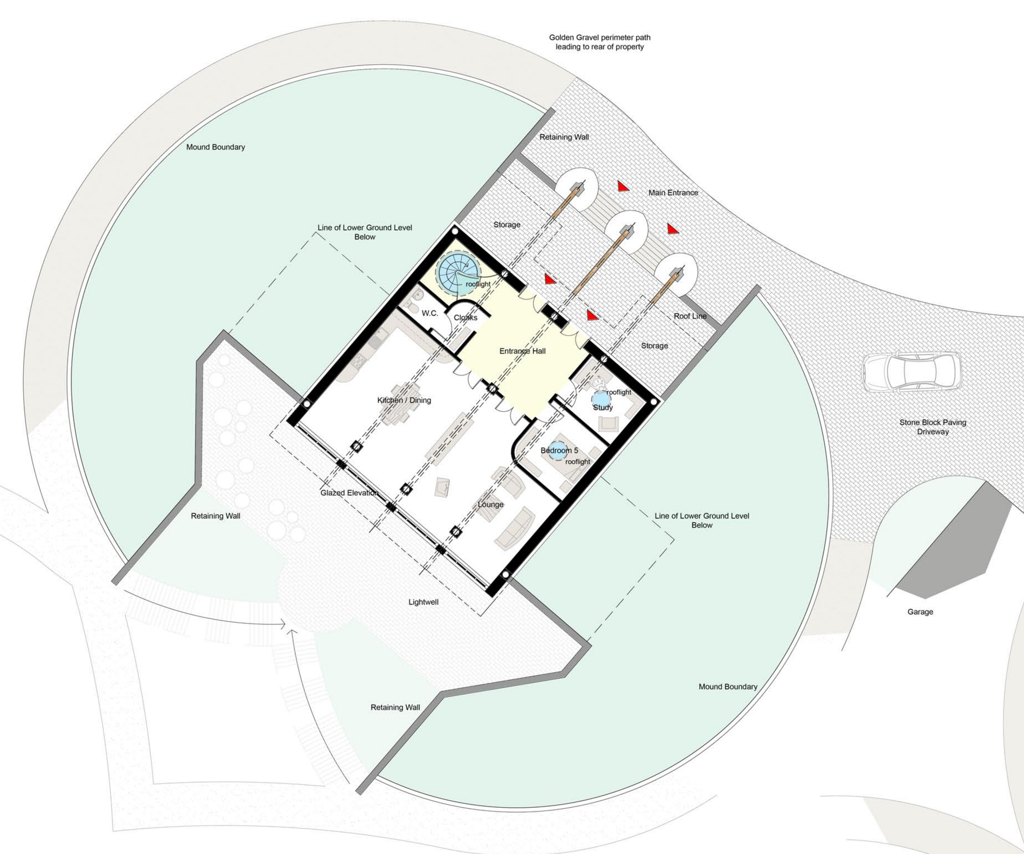
GROUND LEVEL PLAN, SCALE 1:100
