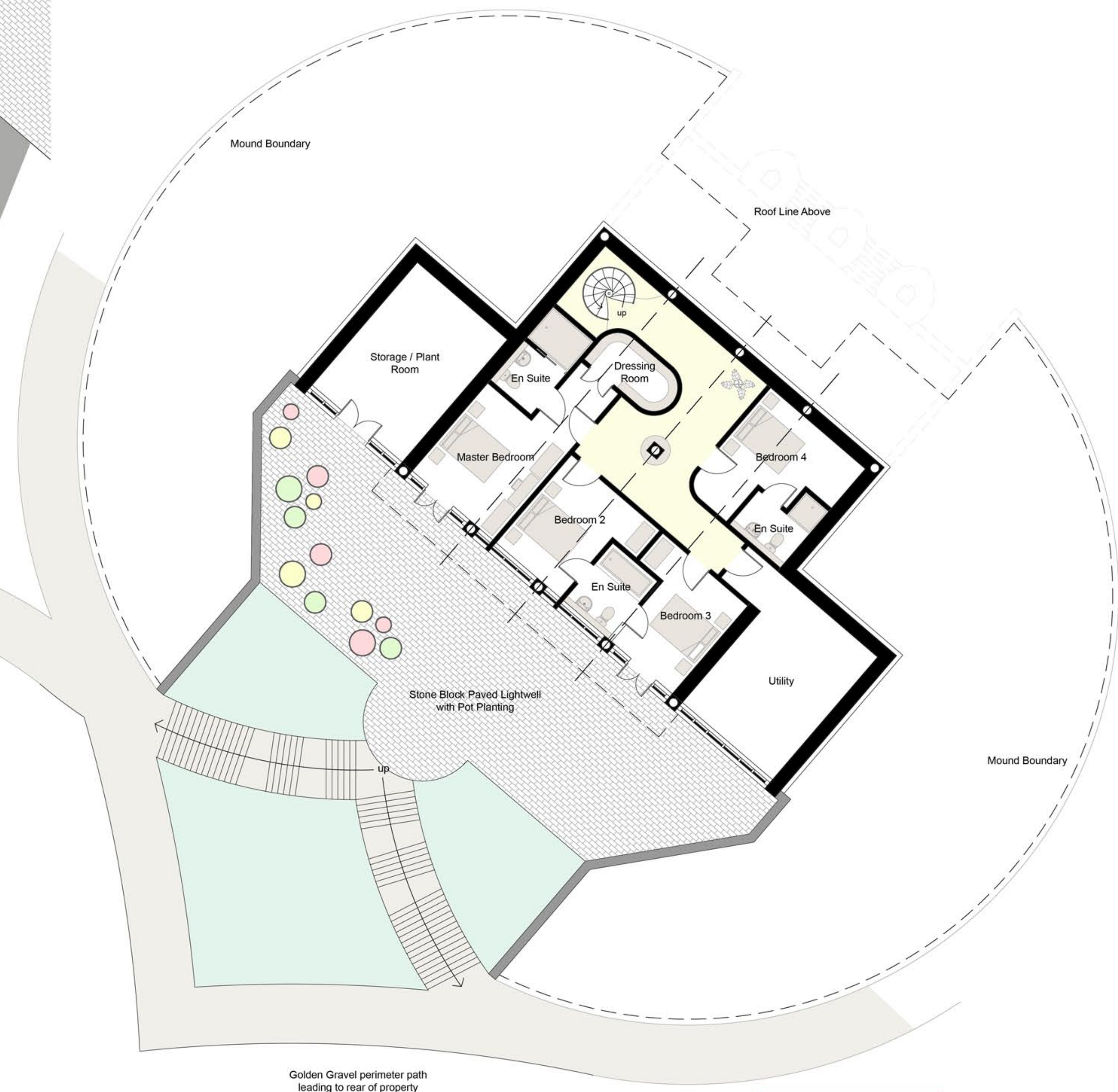
LOWER GROUND LEVEL PLAN, SCALE 1:100
