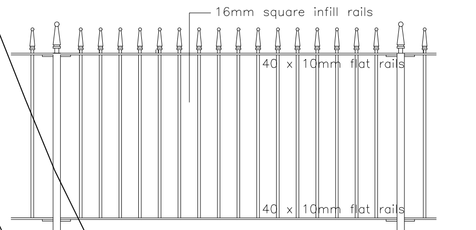
Type 3 1200mm Decorative Top Railing Detail
