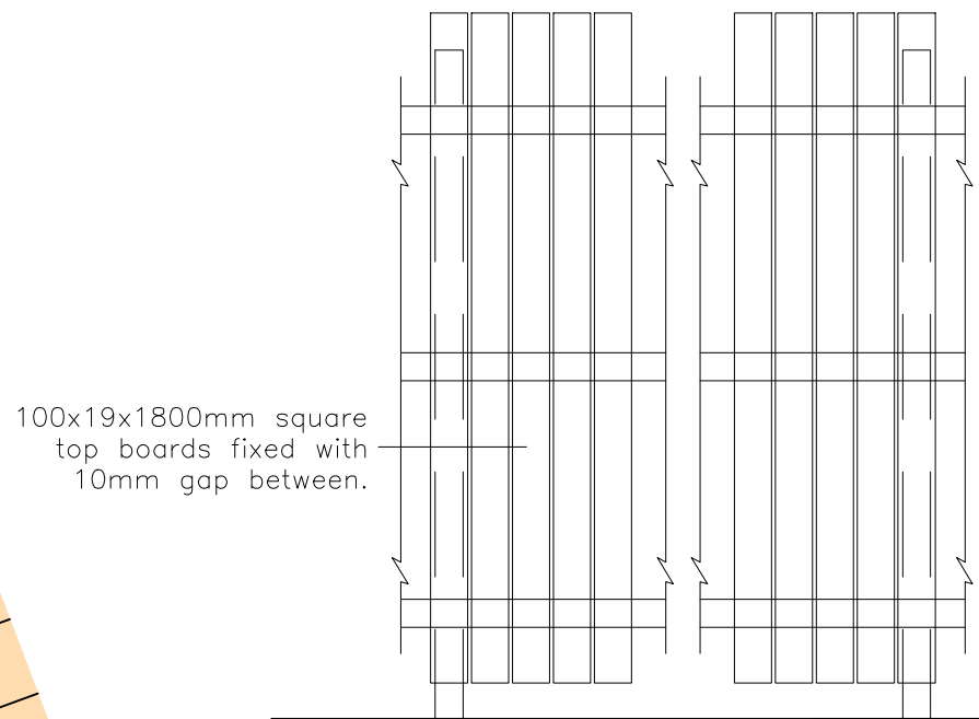
Type 1 Close Boarded Screen Fence
