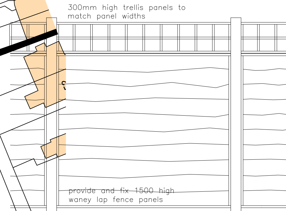
Type 2 Larch Lap/Lattice Fence 1.8m High
