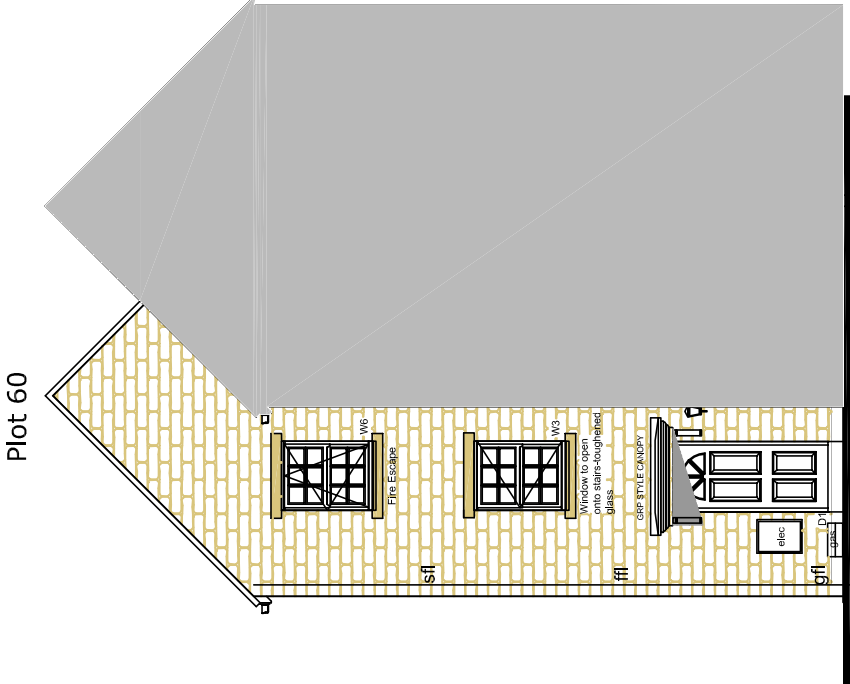
AS (END WITH 45° ROOF) STONE ELEVATION
