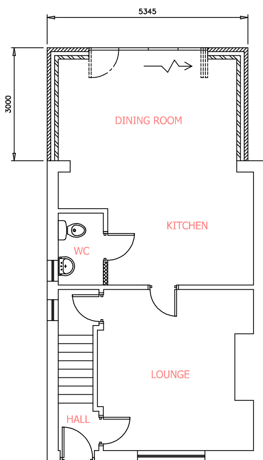
PRO GROUND FLOOR
