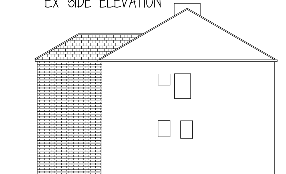
PRO SIDE & REAR ELEVATIONS
