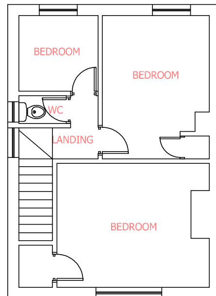
EX FIRST FLOOR
