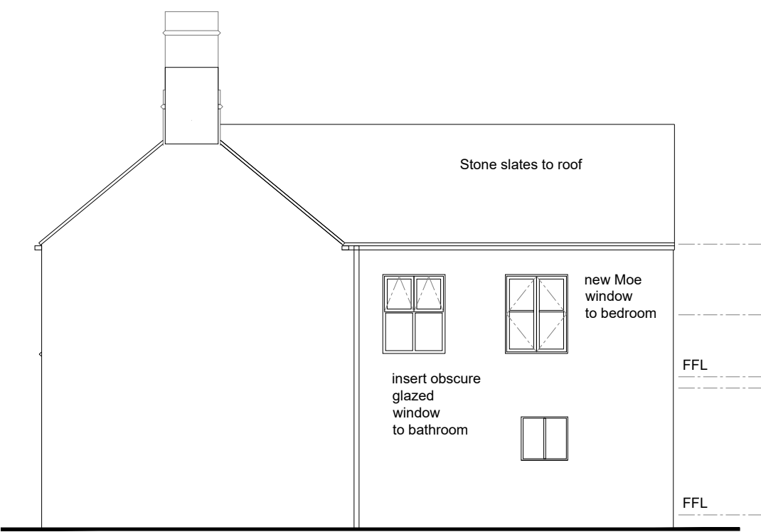
south west (side) elevation
