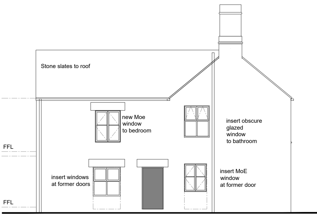
north east (side) elevation
