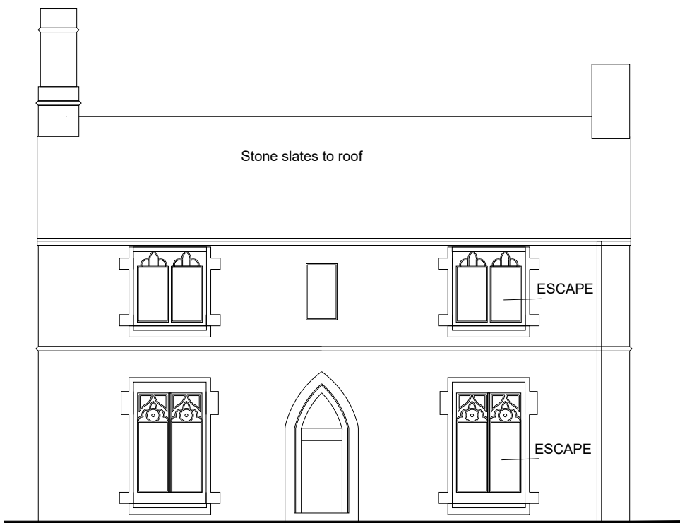
north west (front) elevation
