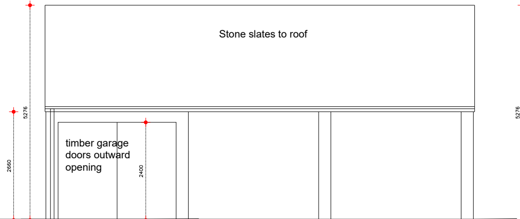
southwest (front) elevation
