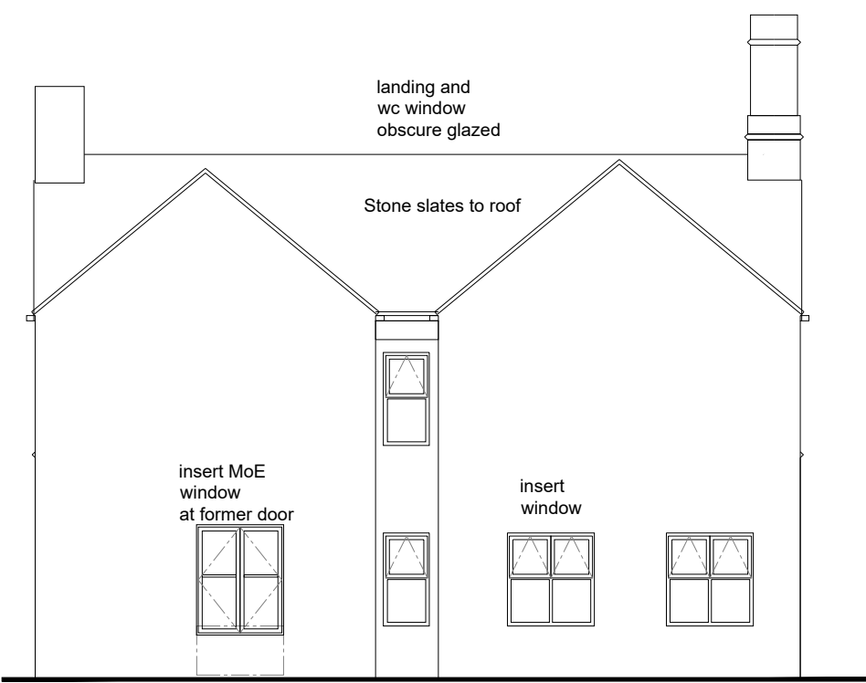
south east (rear) elevation
