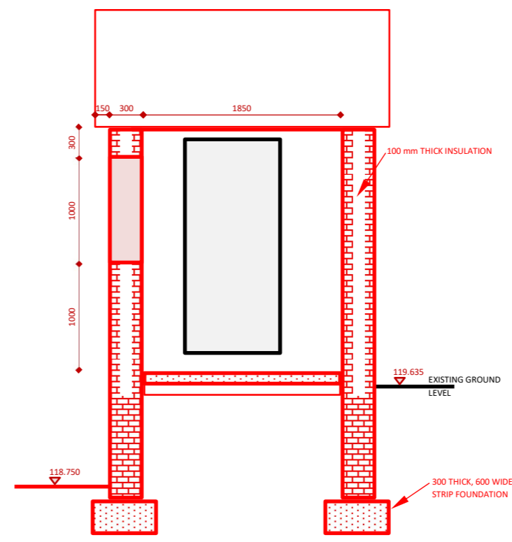
SECTION B-B
