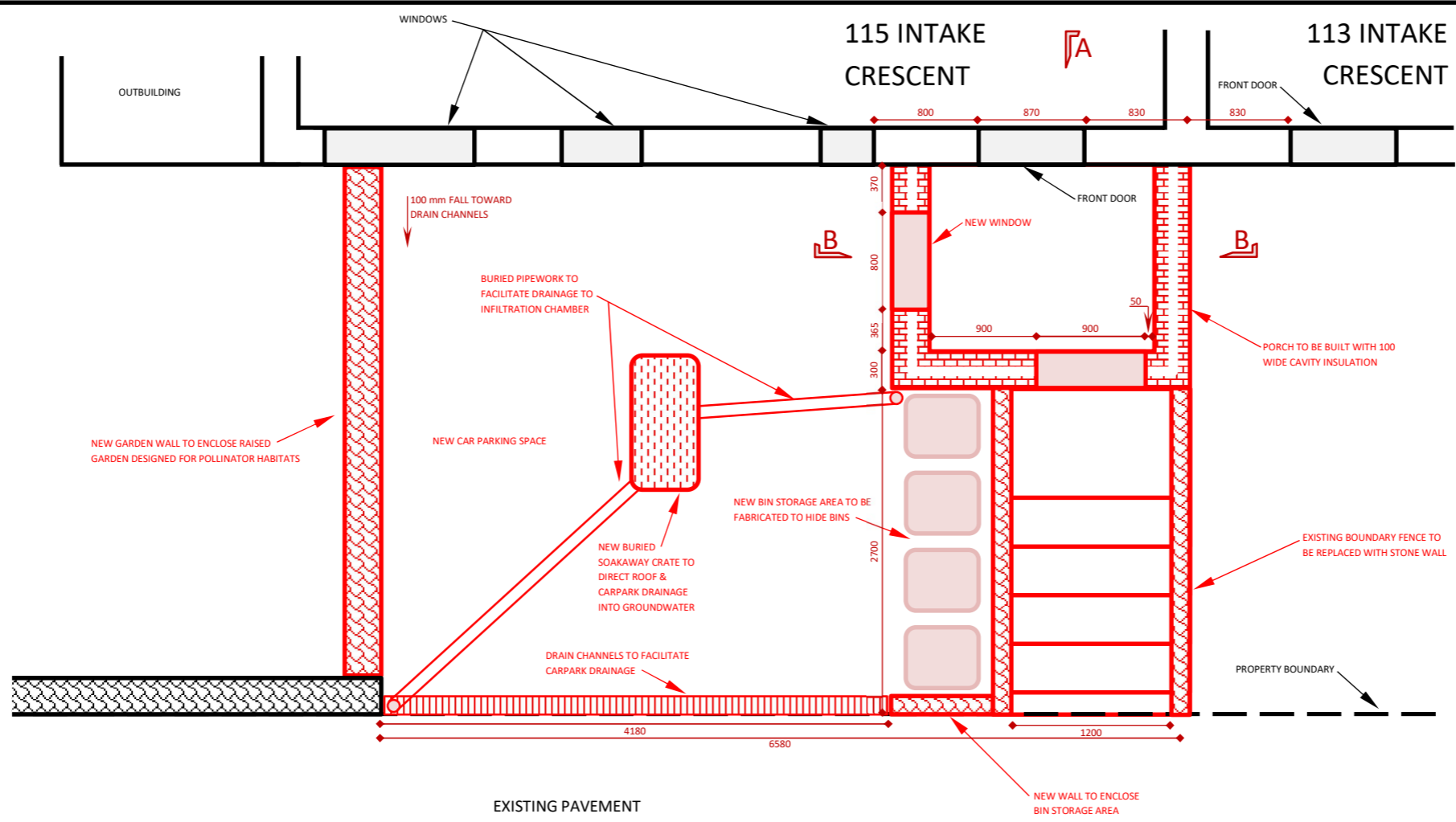
PLAN VIEW
