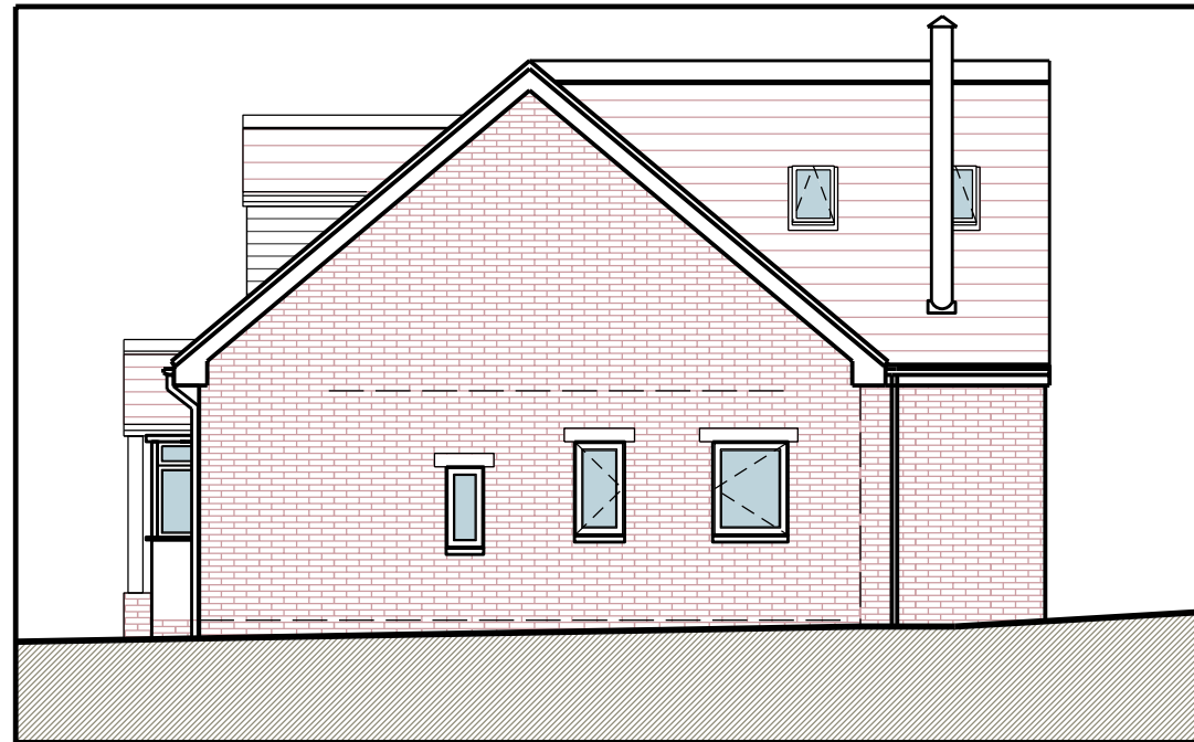
North Elevation
