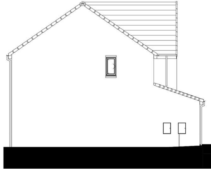
Left Elevation.
