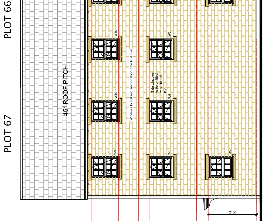
SIDE ELEVATION WITH 45° ROOF STONE ELEVATION
