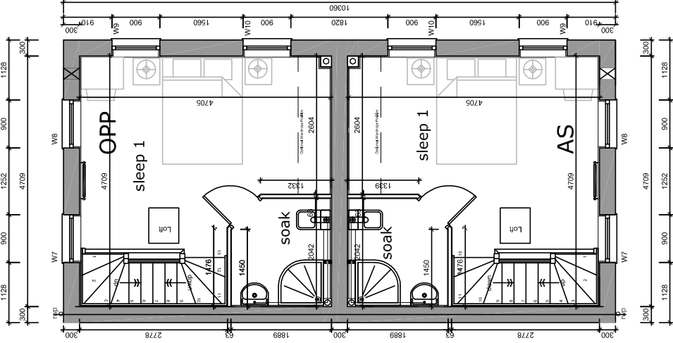
SECOND FLOOR
