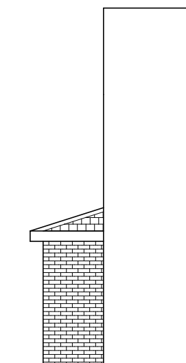
SIDE ELEVATION
