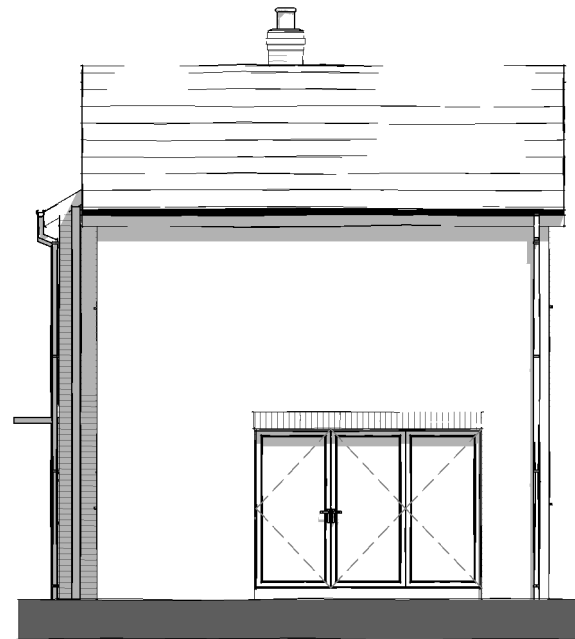
Right Side Elevation. 1 : 100
