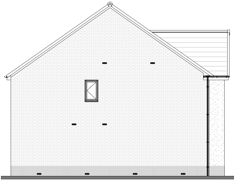
LEFT ELEVATION
