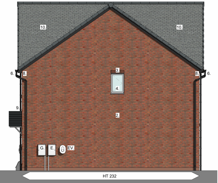
Side Elevation 1 : 100
