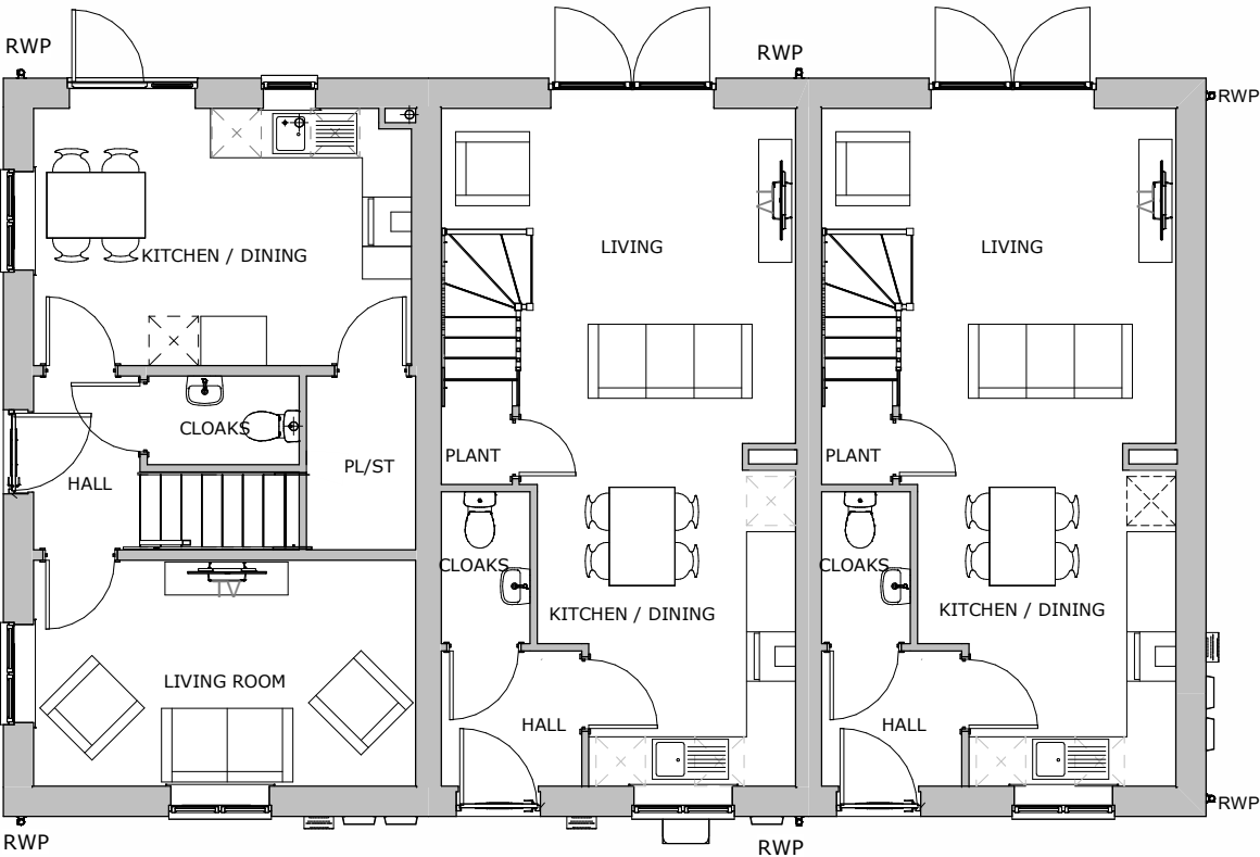
Ground Floor 1 : 100
