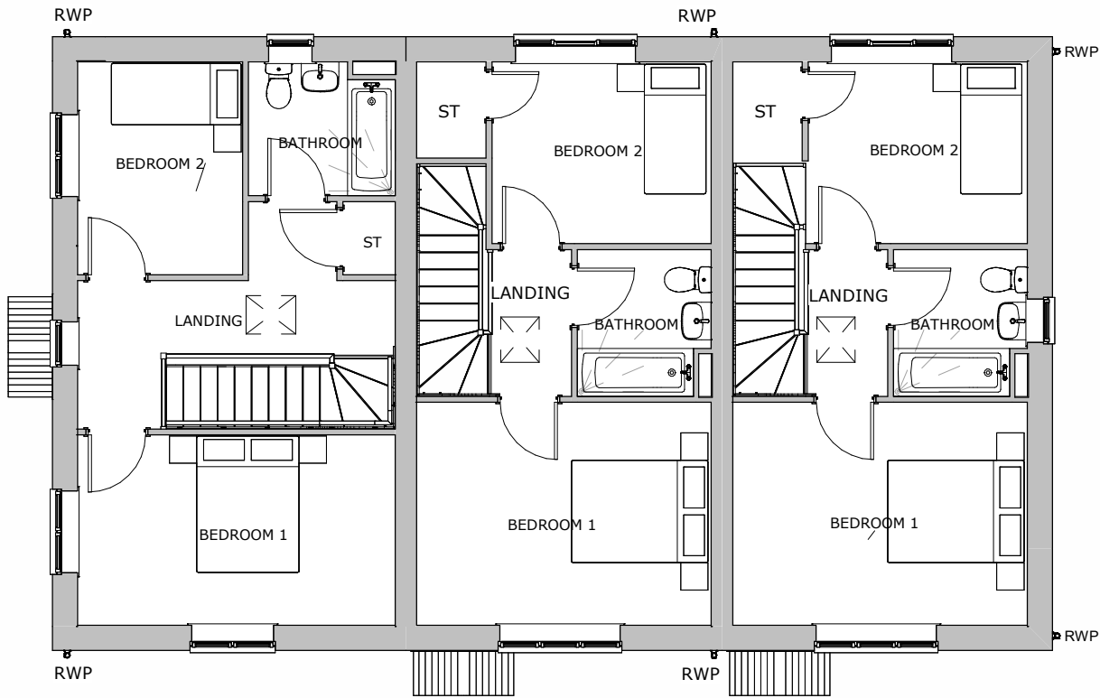
First Floor 1 : 100
