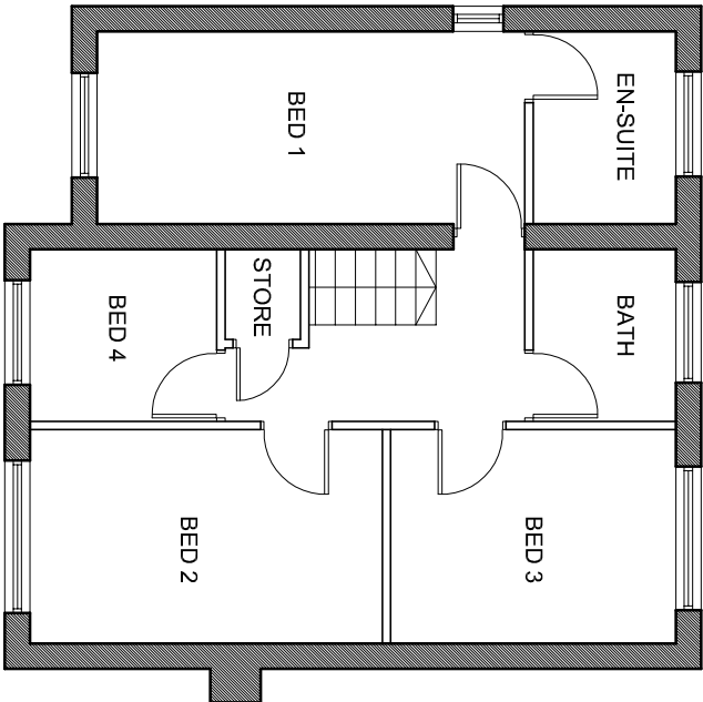
EXISTING FIRST FLOOR PLAN SCALE 1:100
