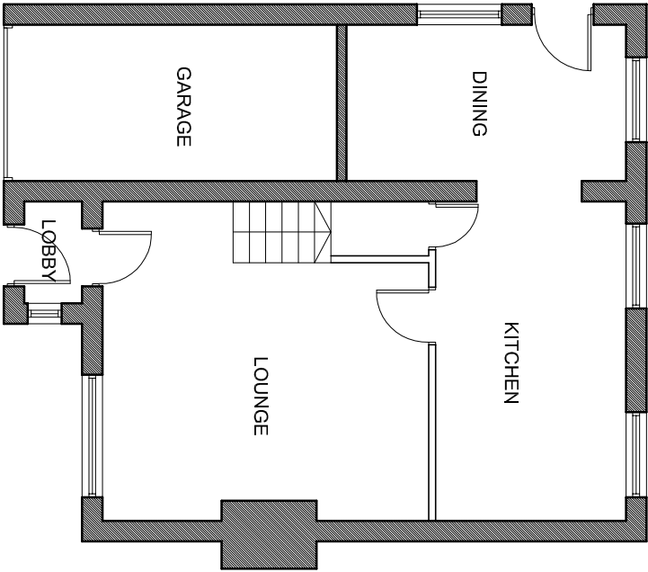
EXISTING GROUND FLOOR PLAN SCALE 1:100
