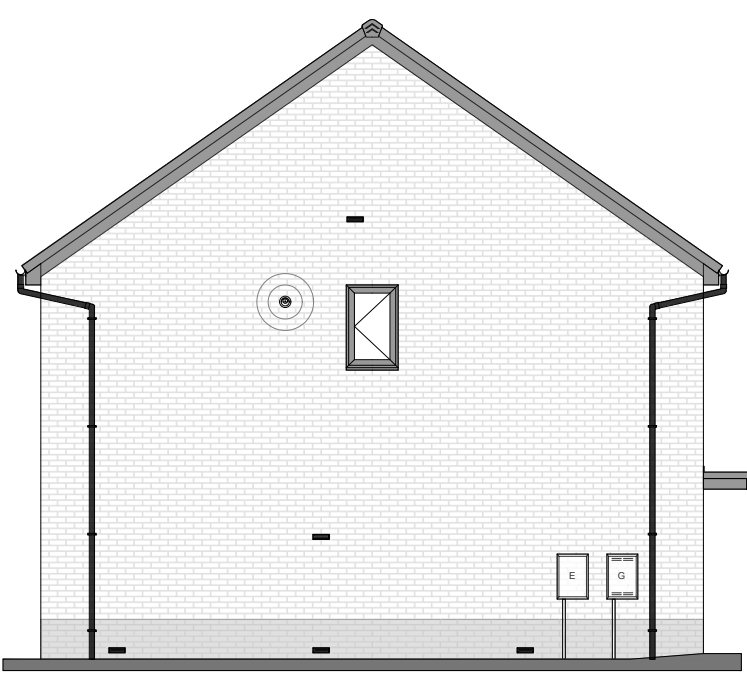
LEFT ELEVATION
